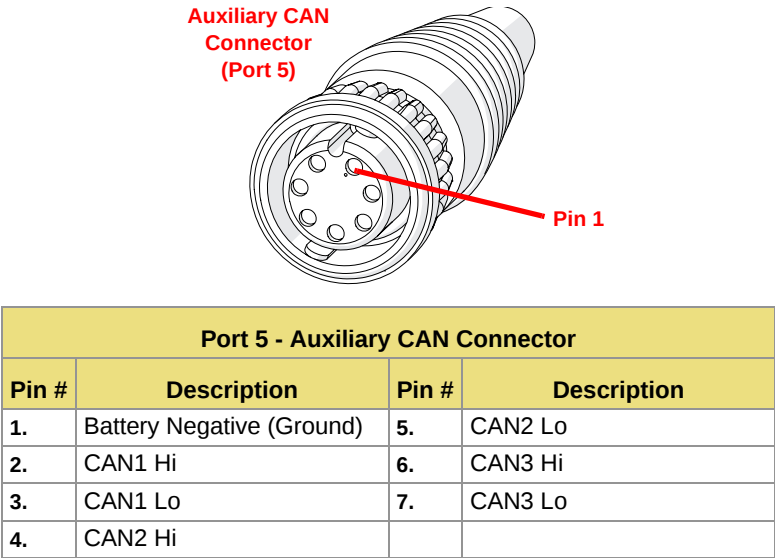
FIGURE 7. Auxiliary CANbus Cable Pin Outs
