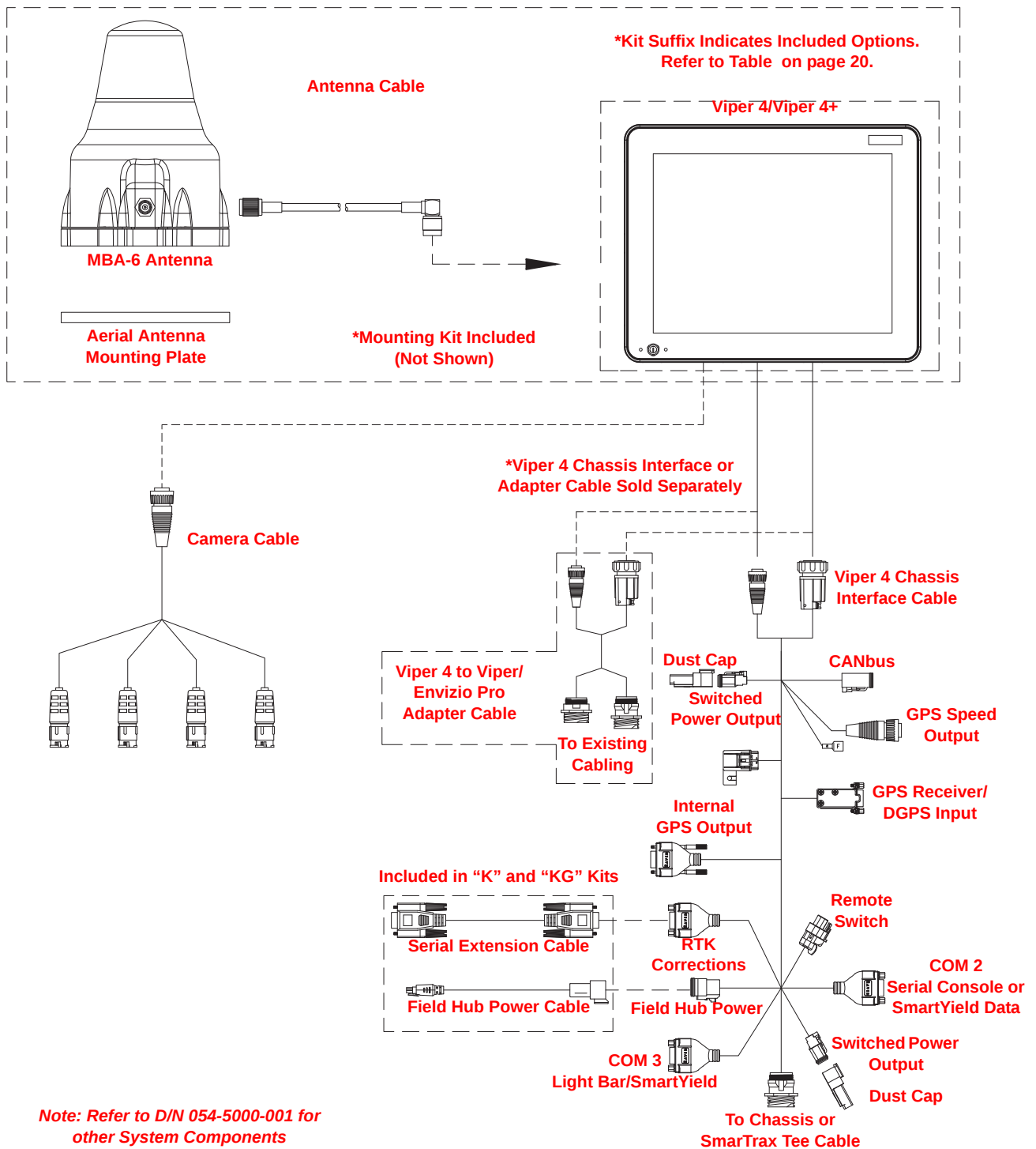
FIGURE 1. Viper 4+ Cable Connections (D/N 054-5010-010)
